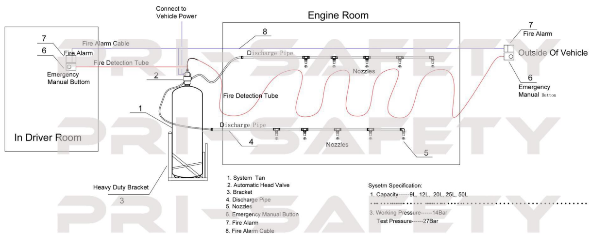
Mining Machine Automatic Fire Suppression Systems
