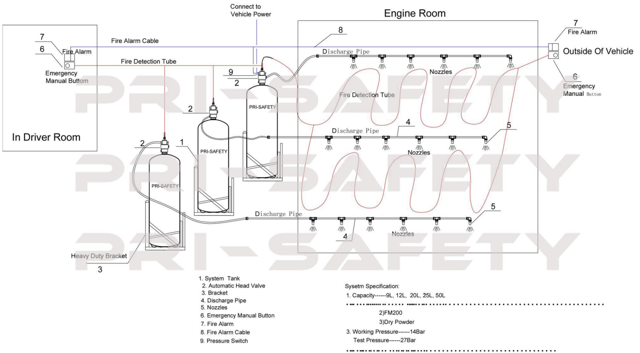
PRI-SAFETY Mining Machine Automatic Fire Suppression Systems
